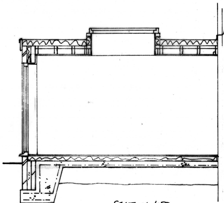
SECTION 1:50
